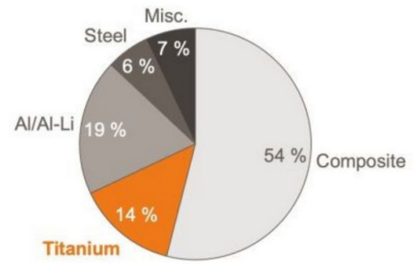
Metal utilization in A350 as % of weight
